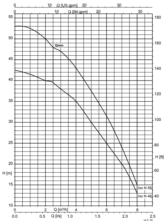
Ixo N 48/58; n = 2900 min -1
